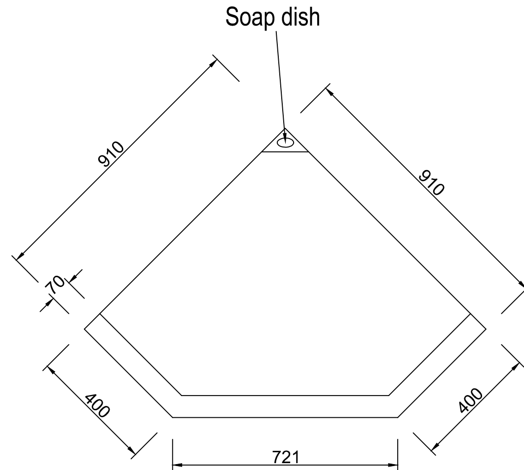
plan view
