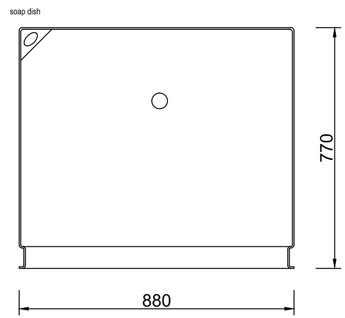
Plan view
